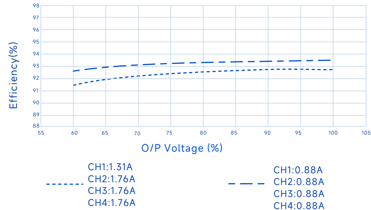
Efficiency Vs. O/P Voltage(Vin=400Vac)
