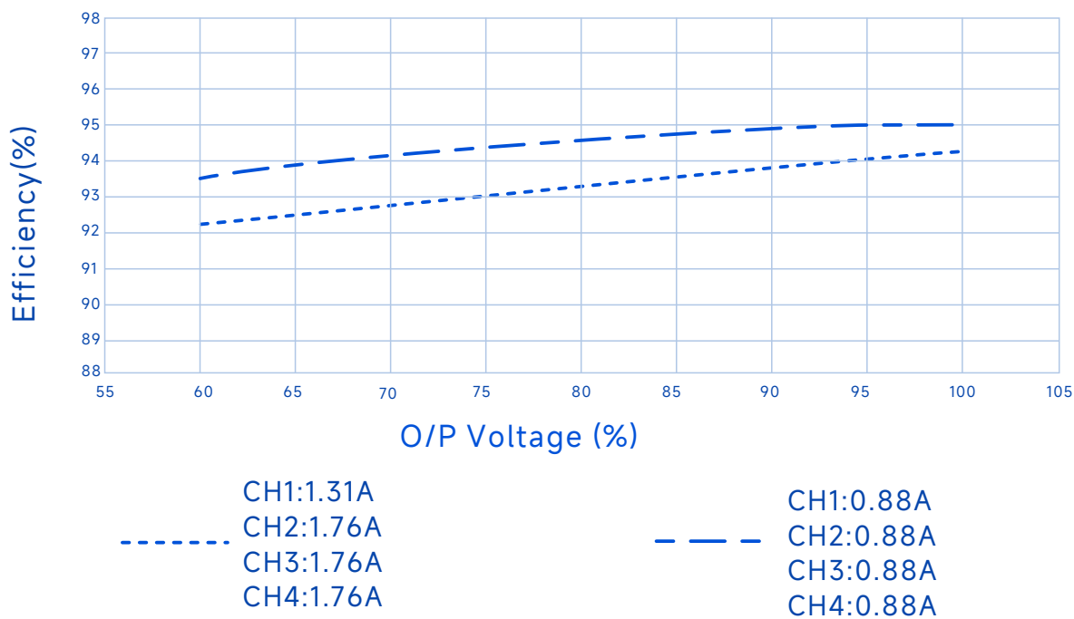
Efficiency Vs. O/P Voltage(Vin=400Vac)
