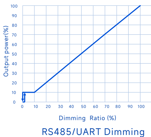
Output Power Vs. Dimming
